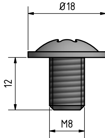
Buttonhead socket screw ISO 7380-2 with torx M8x12mm A4-70
